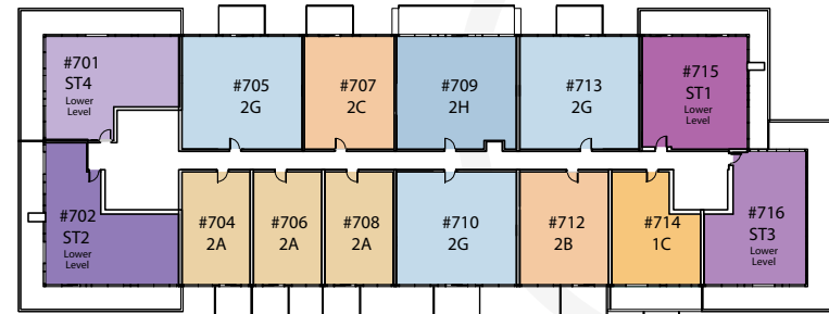
EAST BUILDING
